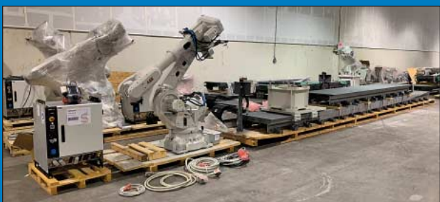
(6) ABB IRB 6700-150/3.20 Six-Axis Track Mounted Robots
